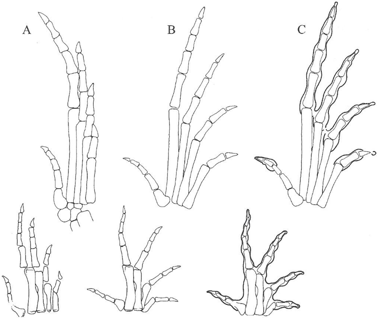
Fig. 9 - Manus and pes of Macrocnemus bassanii specimen BES SC 11 as preserved (A), reconstructed in flat view as semiplantigrade (manus) and digitigrade (pes) configuration (B) and the same reconstructions superimposed to Rhynchosauroides tirolicus ichnites (C)
