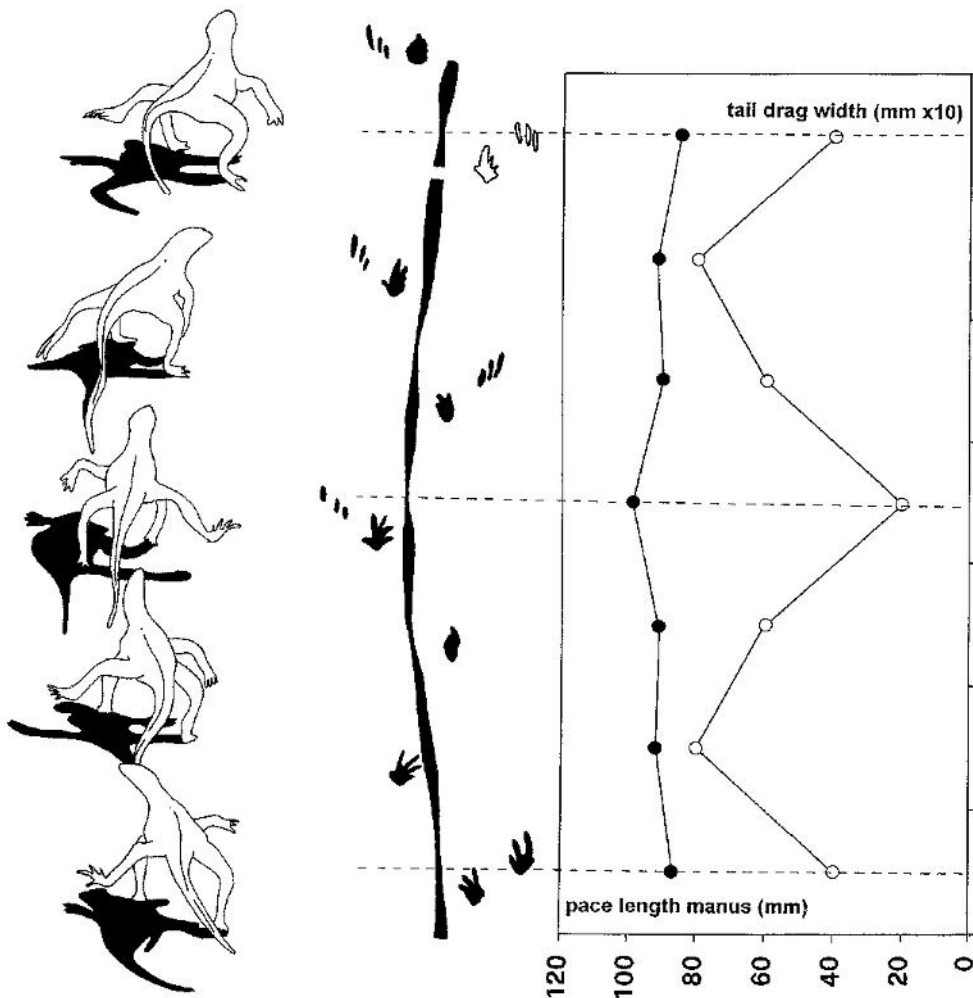
Fig. 4 - Relationships between traces of the tail width and pace length in Rhynchosauroides tirolicus BzULF3/2 trackway. The variation of the width of tail drag is function of the distances of the body of the trackmaker from the surface. This seems related to a gait with brief regular spurts.
