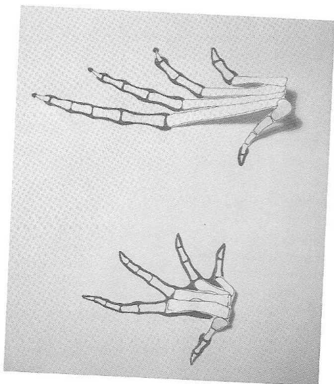
Fig. 10 - Models of Macrocnemus manus (below) and pes (above) reconstructed as semiplandigrade and digitigrade in three dimensional view matching well the traces ascribed to Rhynchosauroides tirolicus .
