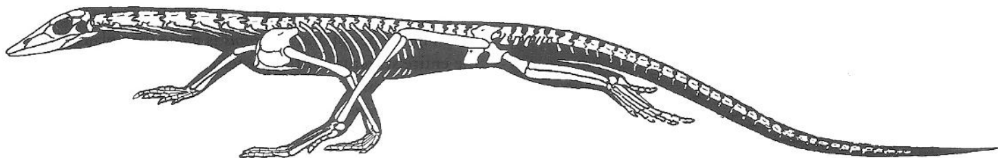
Fig. 11 - Walking Macrocnemus , a possible trackmaker for Rhynchosauroides tirolicus ?
