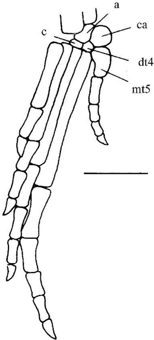
Fig. 6 - Right tarsus and pes of Macrocnemus bassanii , specimen BES SC 11 (Renesto & Avanzini in press). Abbreviations: a) astragalus; c) centrale; ca) calcaneum; dt 4) distal tarsal four; mt5) fifth metatarsal. Scale bar equals 0.5 cm.
