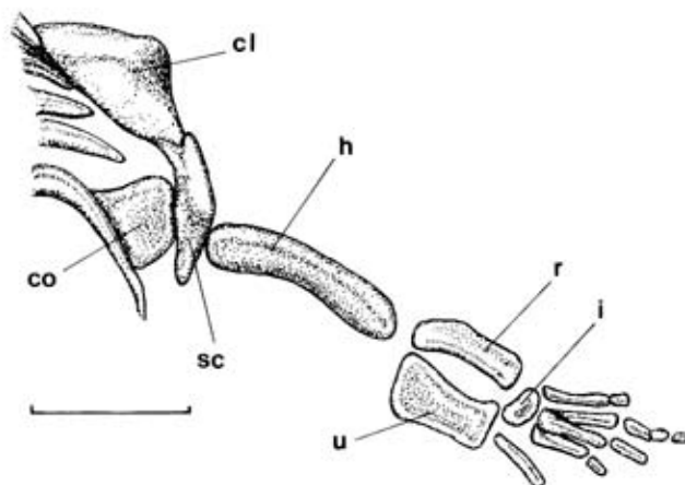
Fig. 2 - The right half of the shoulder girdle and the right anterior limb of specimen 550 MCSNIO, in dorsal view. Abbreviations: cl) clavicle; co) coracoid; h) humerus; i) intermedium; r) radius; sc) scapula; u) ulna. Scale bar equals 1 cm.
