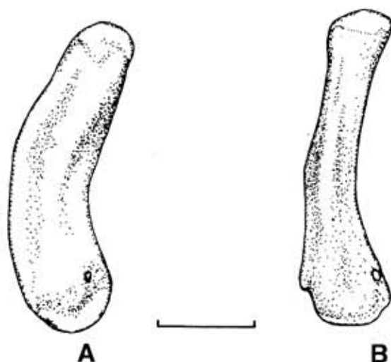
Fig. 4 - Morphological comparison of different lariosaur humeri. A) L. balsami , Munich specimen (after Peyer, 1933); B) L. valceresii , holotype (after Tintori & Renesto, 1990). Scale bar equals 2 cm.
